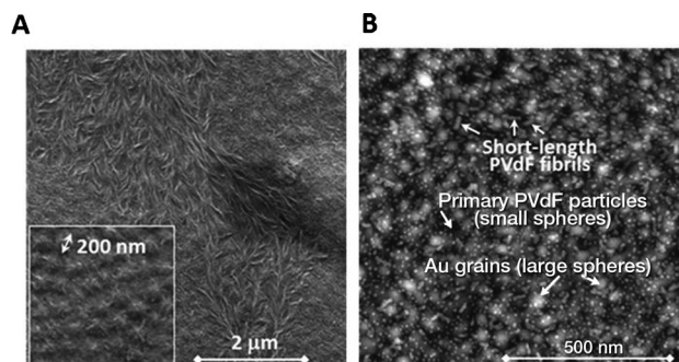
Figure 2. SEM (A) and AFM (B) images of neat PVdF coating on a quartz crystal obtained from concentrated and diluted solutions, respectively, revealing the multiscale character of the polymer film morphology.
