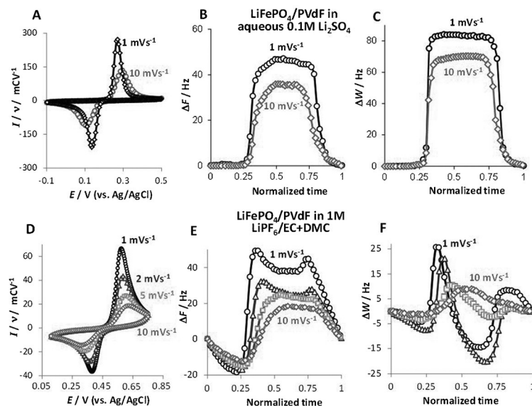
Figure 4. CVs at different scan rates as indicated and the related changes in the experimental frequency, \Delta F , and the resonance width, \Delta W , of the QC during charging–discharging cycles of \text{LiFePO}_4/\text{PVdF} electrodes in 0.1 M aqueous \text{Li}_2\text{SO}_4 (A–C) and 1 M \text{LiPF}_6/\text{EC} + \text{DMC} (D–F).
